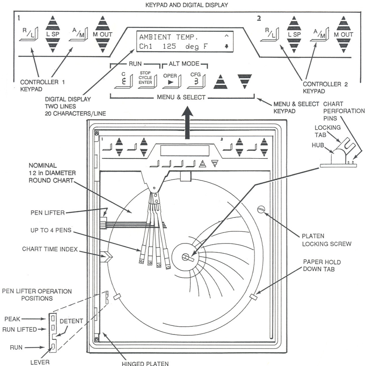
Figure 1. Controller with Front Door Removed
